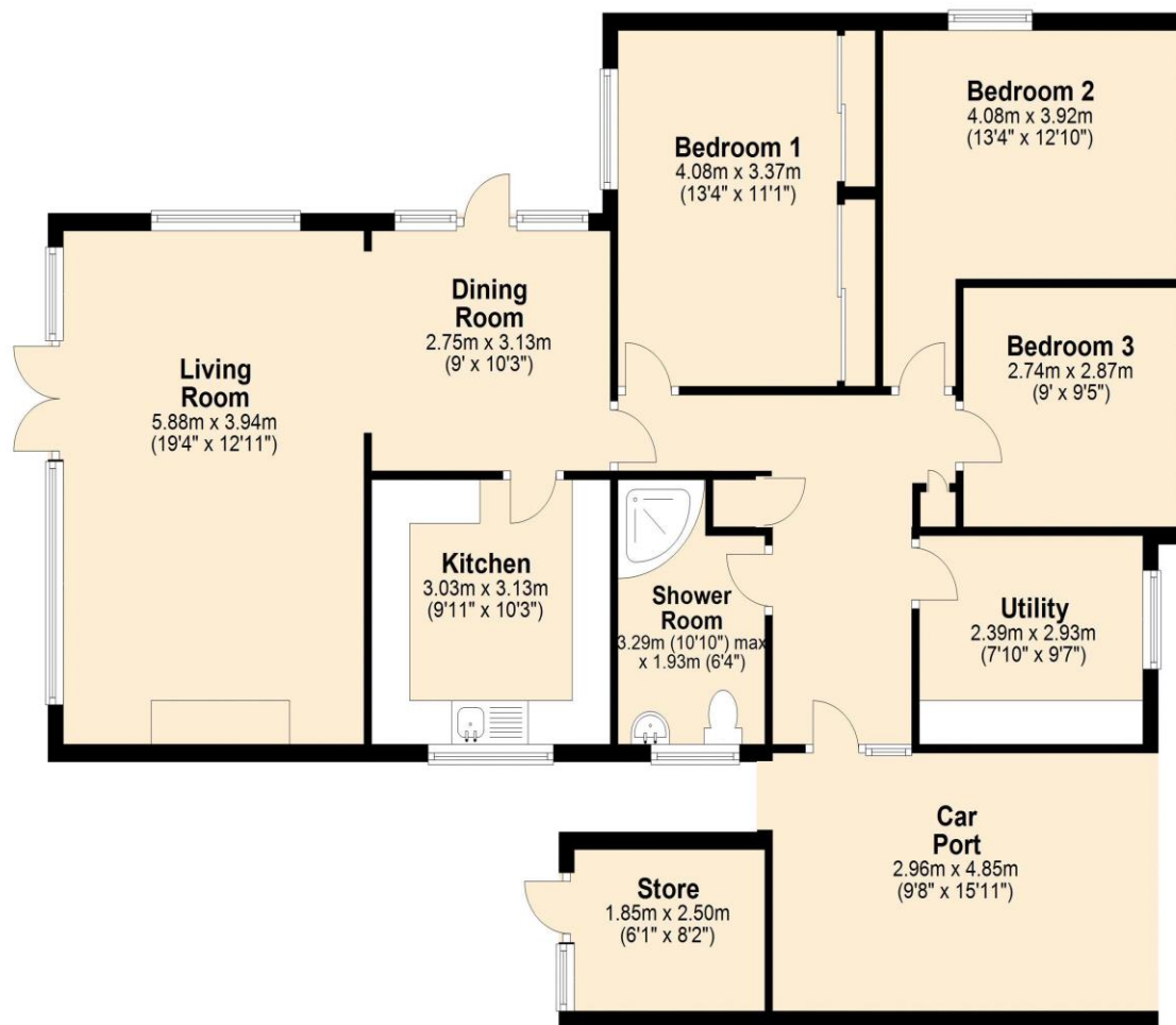
Ground Floor Approx. 121.8 sq. metres (1311.3 sq. feet)
